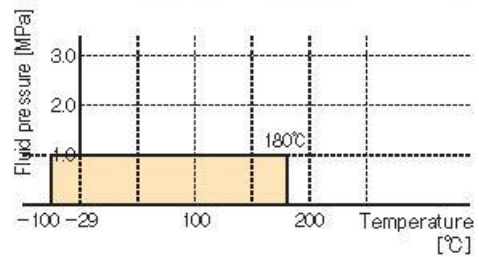
Gas-type fluid
